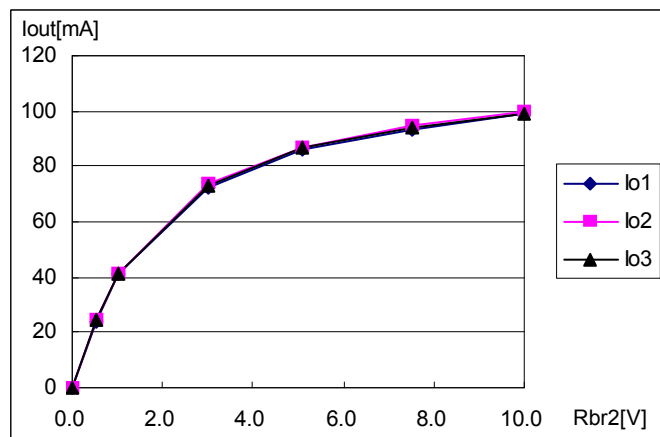
Fig.5-7 Current Resistor Dimming Characteristics(Rbr2 vs Iout)
