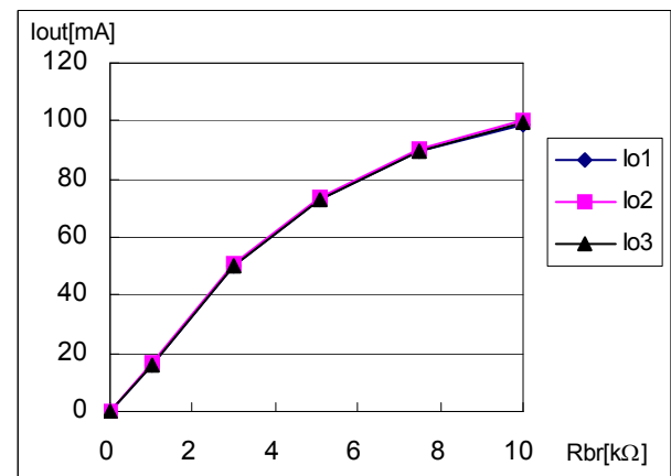
Fig 5-5 PWM Resistor Dimming Characteristics(Rbr1 vs Iout)
