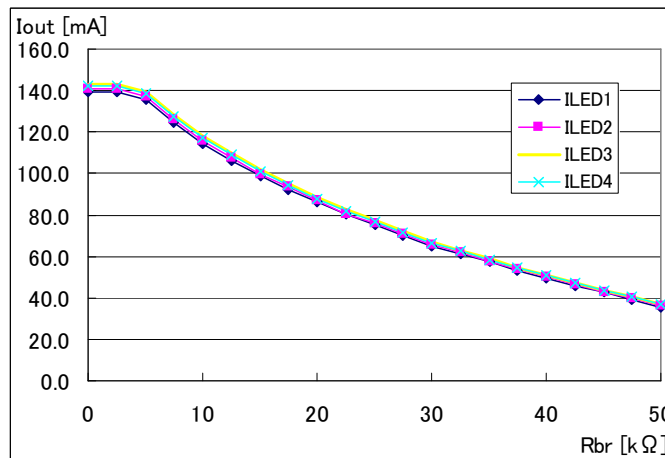
Fig. 5-9 PWM Resistor dimming characteristics(Rbr vs Iout)
